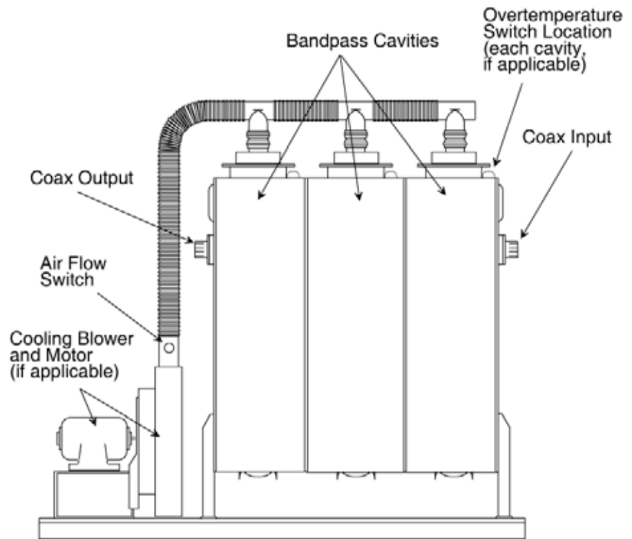
Figure 1. Typical Bandpass Filter, Front View
