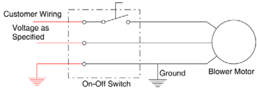
Figure 2. Blower Motor Wiring
