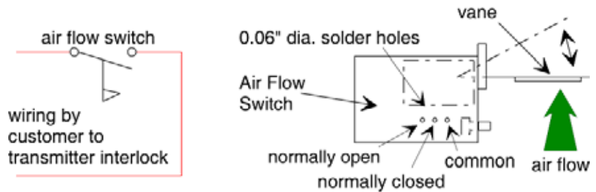
Figure 3. Air Flow Switch Wiring
