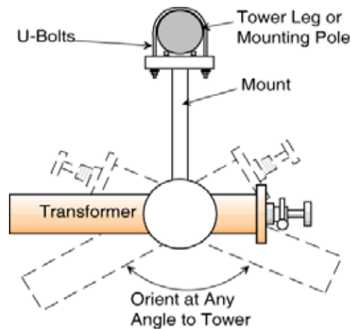
Figure 8. Transformer Installation, top view
