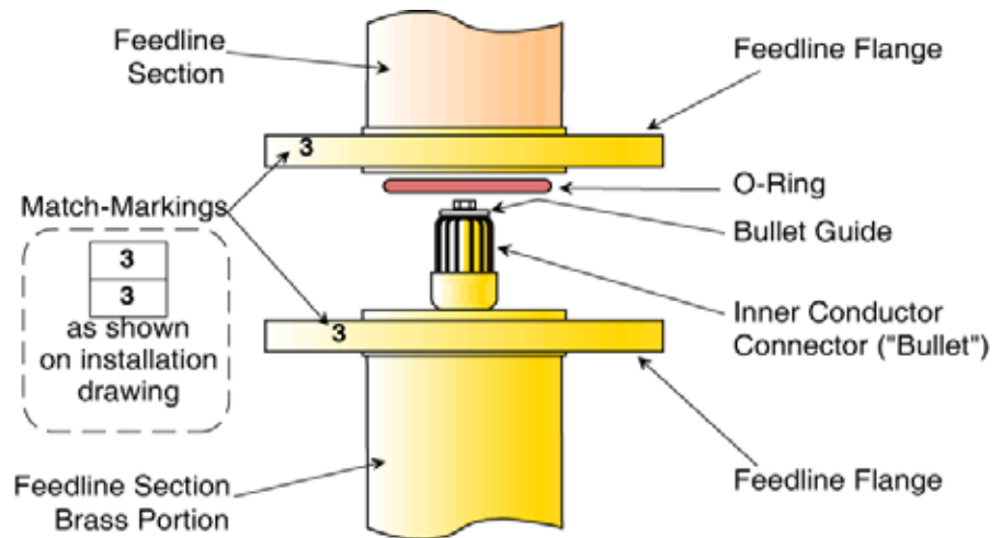
Figure 5. Feedline Flange Detail
