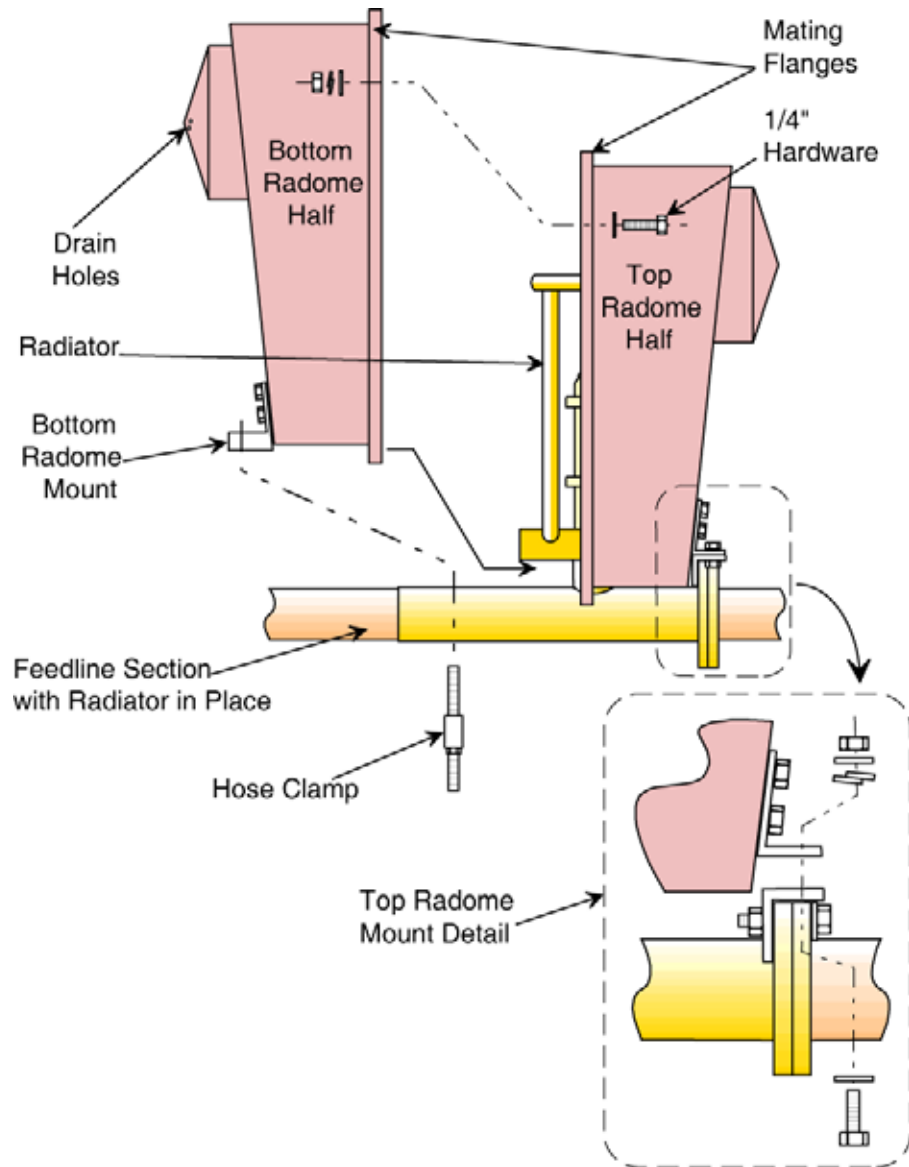
Figure 4. Radome Installation
