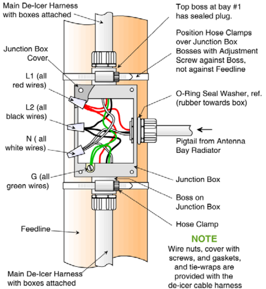
Figure 10. Bay Junction Box Installation
