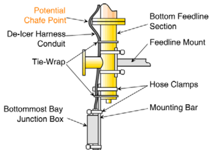
Figure 10. Bay Junction Box Installation
