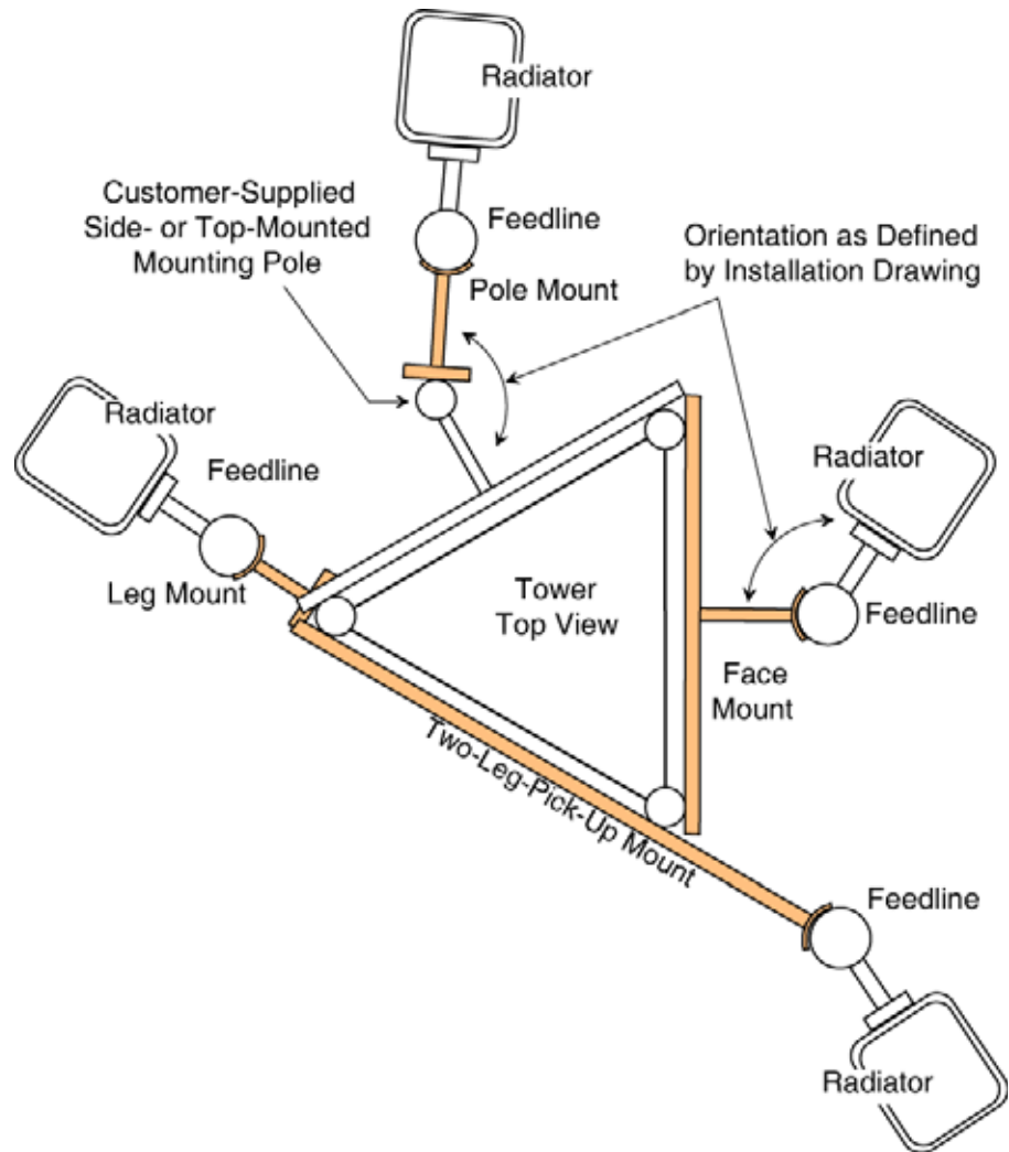
Figure 6. Common Mounting Styles
