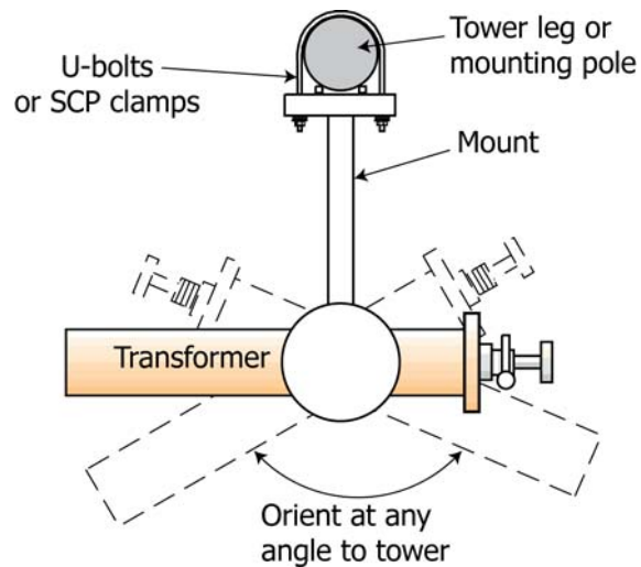
Figure 10. Transformer Installation, top view
