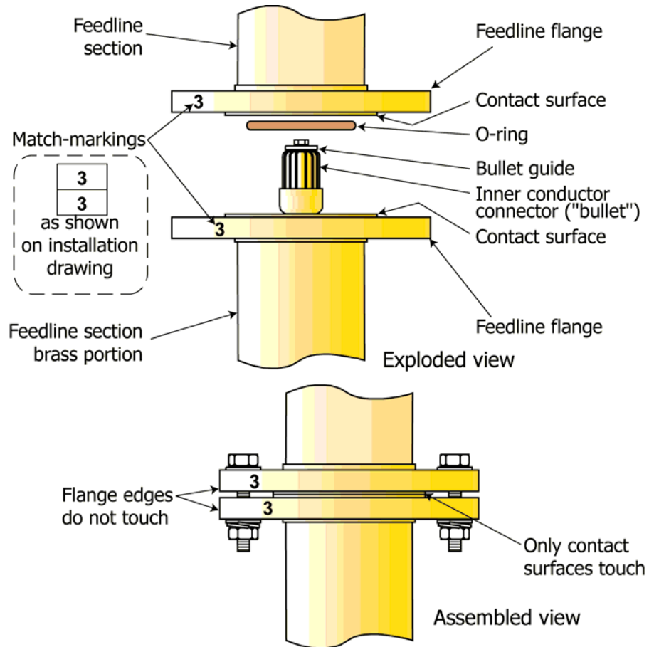
Figure 9. Feedline flange detail
