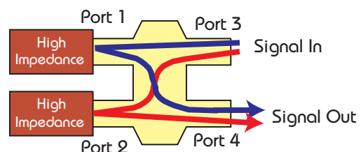
Fig. 5C Hybrid Used as a Signal Reflector
