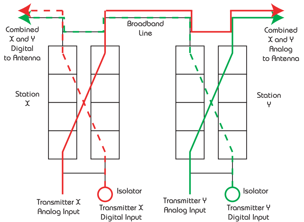
Figure 2. Back-feed Configuration
