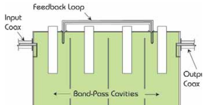
Figure 12. Typical Cross-Coupled Filter Construction
