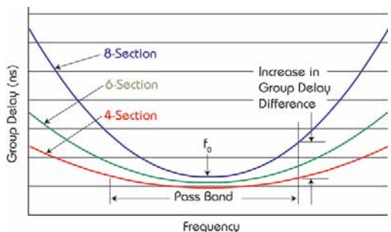
Figure 6. Group Delay Difference Increases with Additional Resonant Sections
