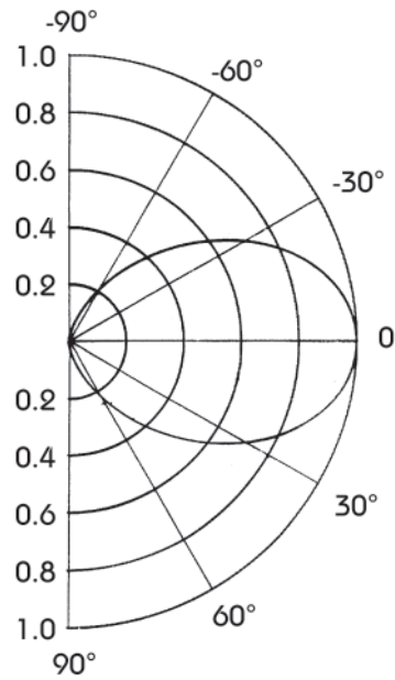
Figure 4b. Elevation Pattern, Two-Element Half-Wave-Spaced Array
