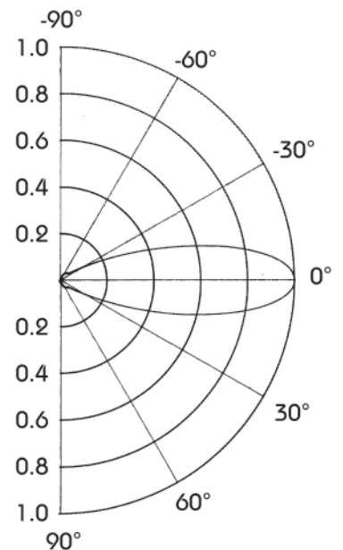
Figure 21. Field Elevation Pattern Plot, Six-Bay Half-Wave-Spaced Array Gain = 1.41
