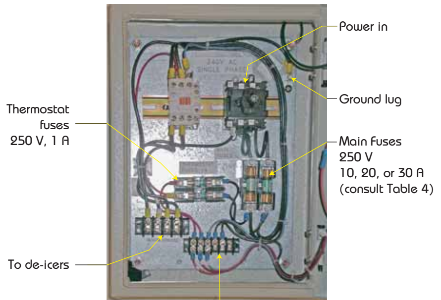
Bay Junction Box
