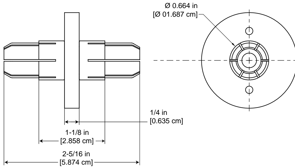
1-5/8" EIA Anchor Connector Assembly Part No. 158F-501
